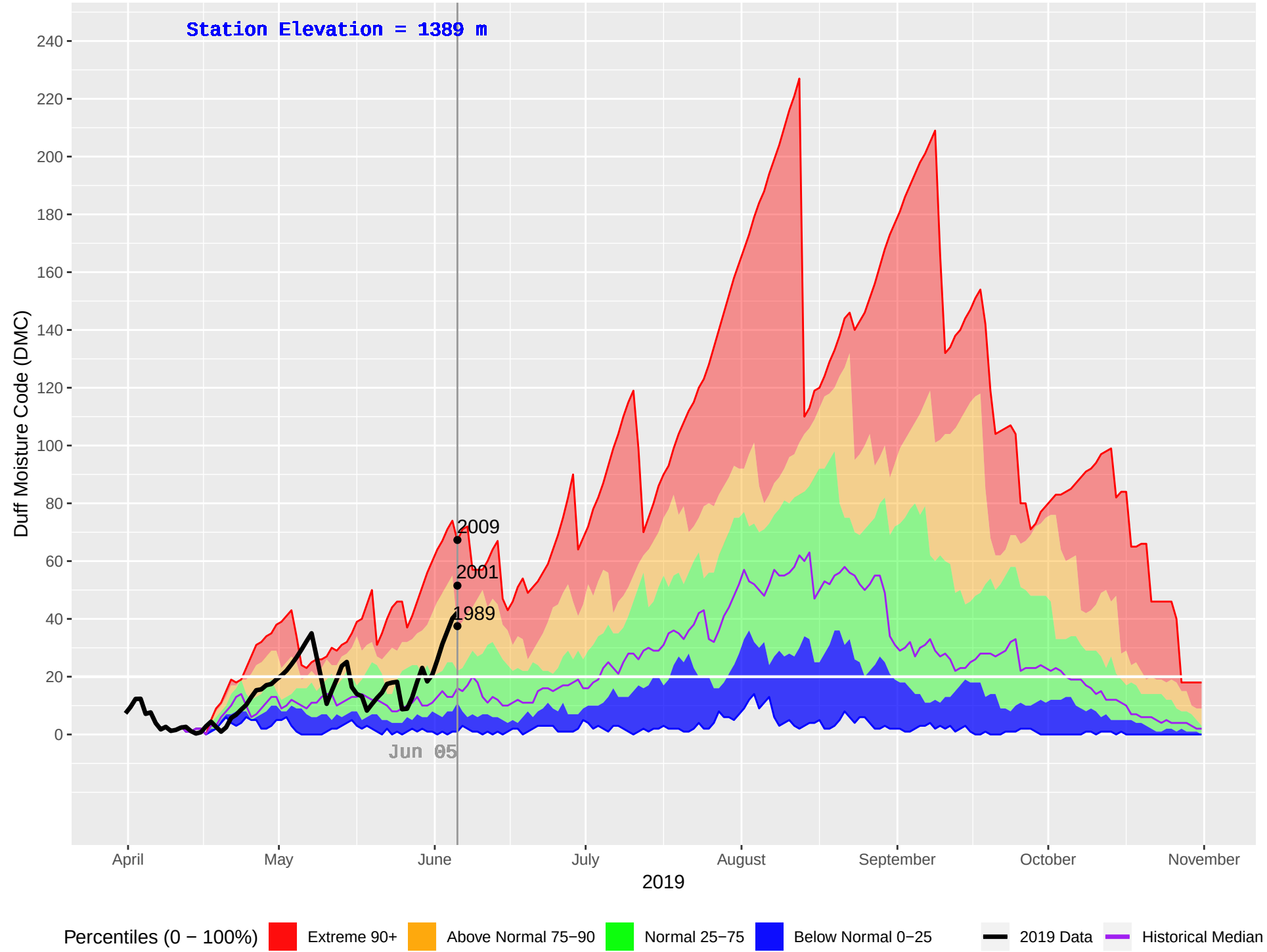
KETTLE 2 (388) : Historical (1987–2018), Current (2019) Daily Duff Moisture Code (DMC)
