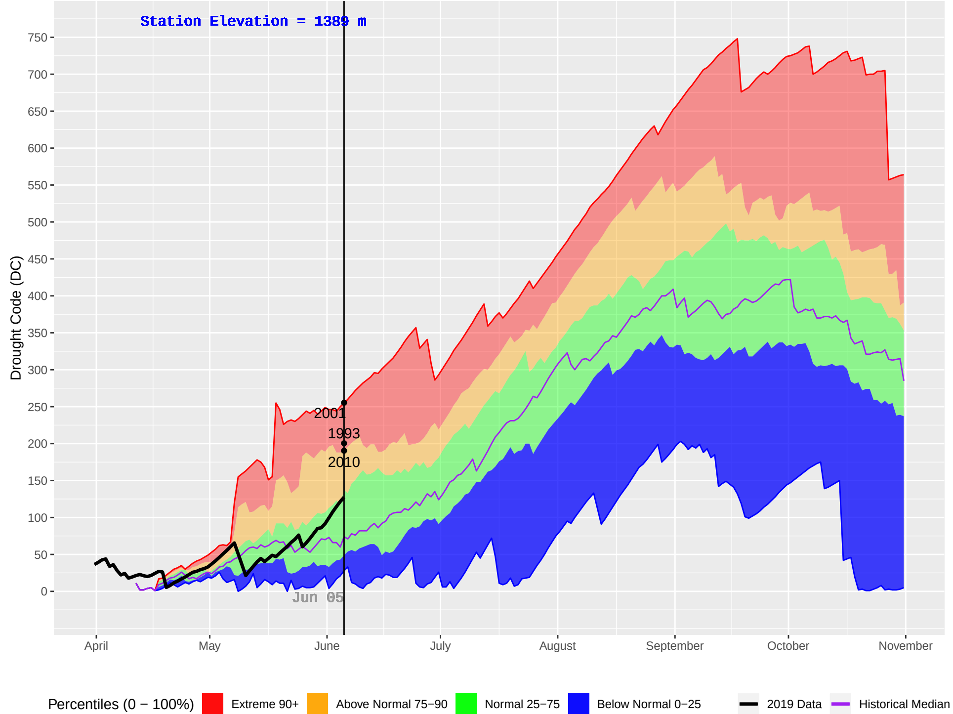
KETTLE 2 (388) : Historical (1987–2018) and Current (2019) Daily Drought Code (DC)
