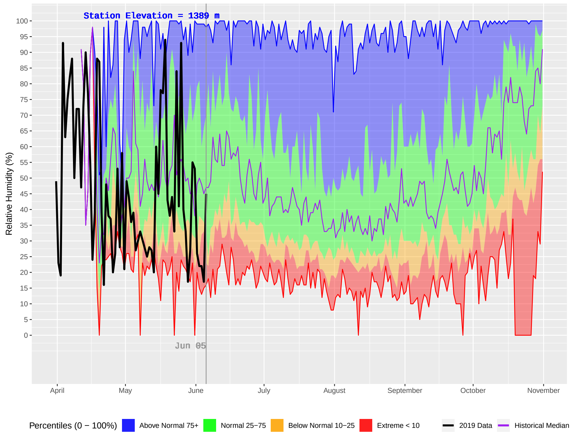
KETTLE 2 (388) : Historical (1987–2018) and Current (2019) Daily Relative Humidity
