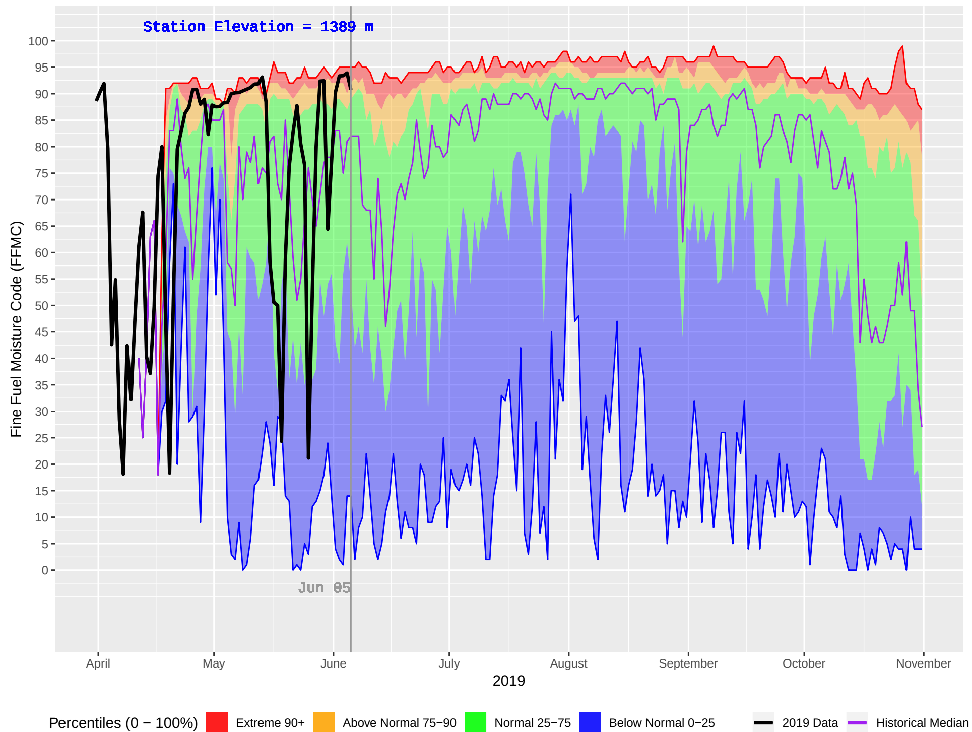
KETTLE 2 (388) : Historical (1987–2018) and Current (2019) Daily Fine Fuel Moisture Code (FFMC)
