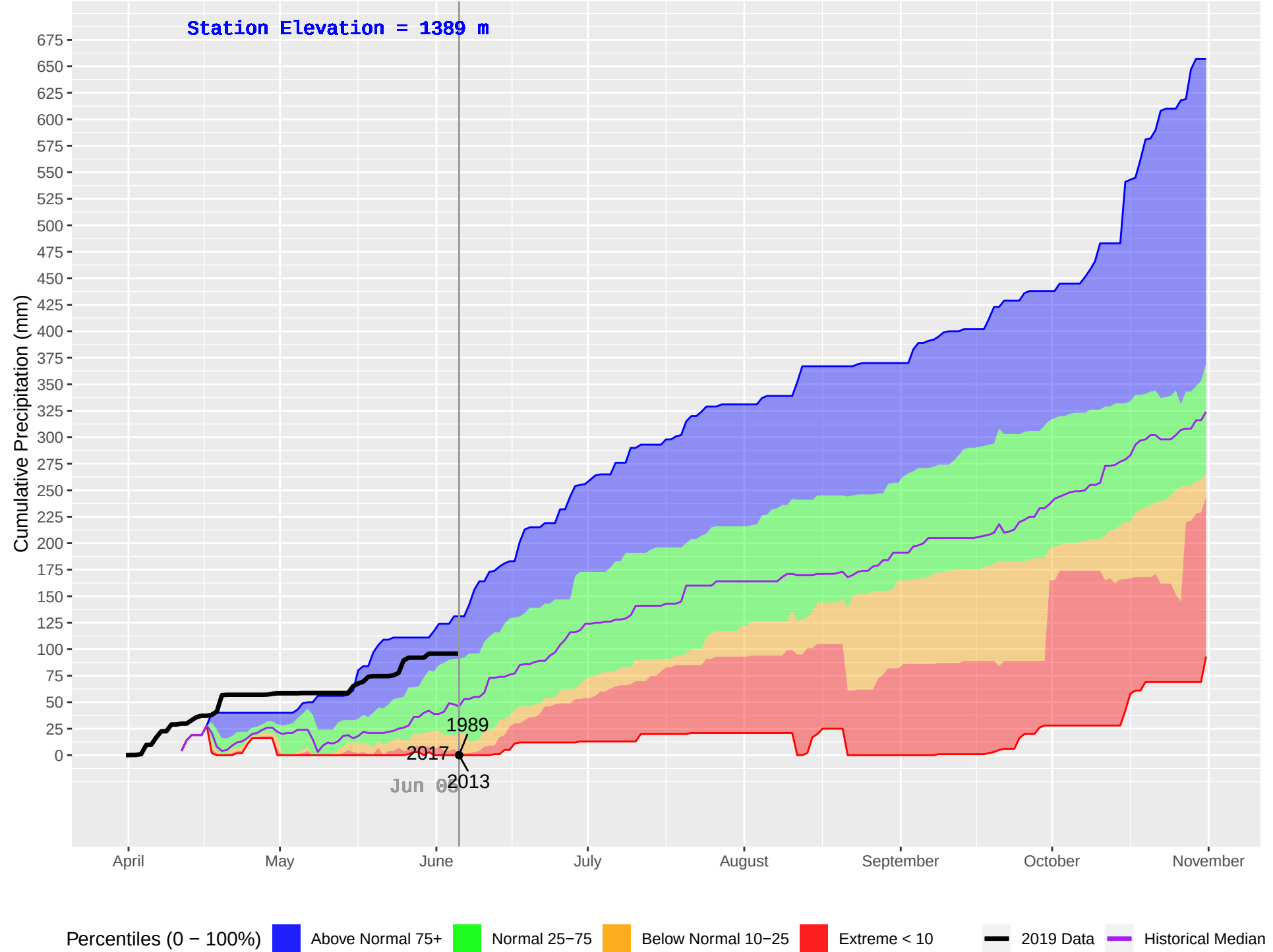
KETTLE 2 (388) : Historical (1987–2018), Current (2019) Daily Cumulative Precipitation
