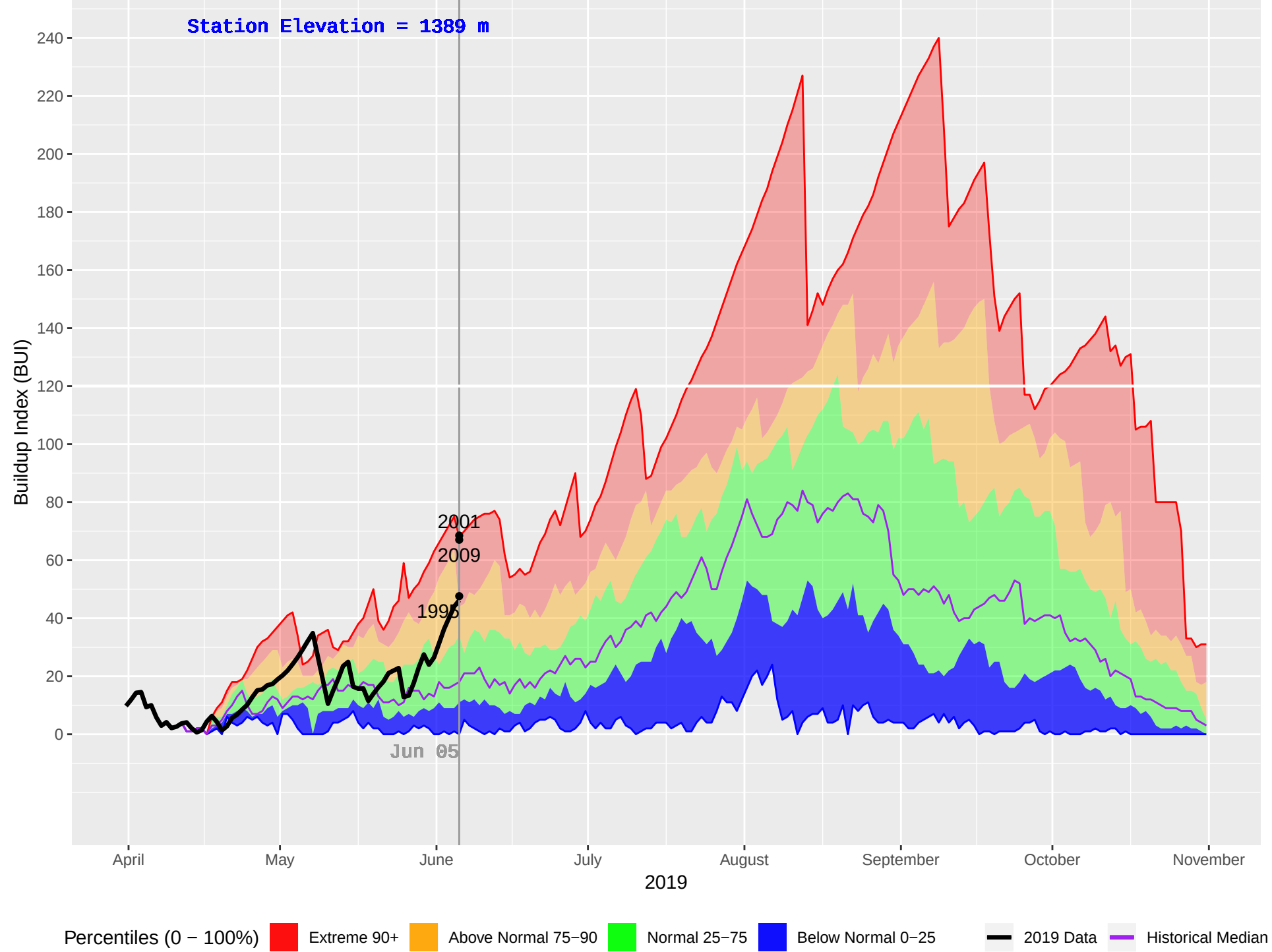
KETTLE 2 (388) : Historical (1987–2018), Current (2019) Daily Buildup Index (BUI)
